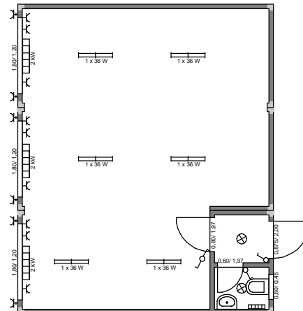
ARS DR4 - 7.31m x 6.05m RH 2.50m
