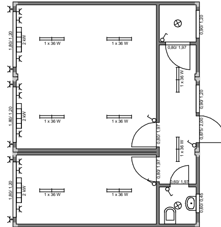
ARS DR2 - 7.31m x 6.05m RH 2.50m
