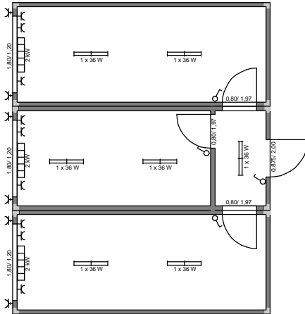
ARS DR1 - 7.31m x 6.05m RH 2.50m
